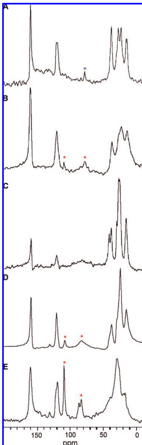
Figure 5. Solid-state ^{13}\text{C} NMR spectra of cococrystals: (A) cococrystal 4\cdot 1 ; (B) cococrystal 4\cdot 2 ; (C) black cococrystals prepared with host 5 ; (D) cococrystals from panel C after being heated under vacuum at 30\text{ }^\circ\text{C} for 1 month; and (E) gold cococrystals with host 6 . Blue asterisks mark the peak for monomer 1 ; red asterisks mark signals for PIDA 2 .
