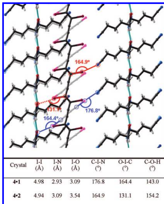
Figure 4. The lighter background shows the structure of the monomer diiodobutadiyne cocrystal; the bold foreground drawing shows the structure of the resulting PIDA. The symbols in the figure represent the halogen bond angle changes between guest and host (blue, monomer; red, polymer; dashed line, pointing out of the plain). The table below summarizes the changes in the crystal structure upon polymerization.
