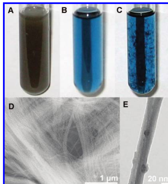
Figure 10. Suspensions and aggregates of PIDA. (A) Gold 6•2 cocrystals dispersed in \text{H}_2\text{O} . (B) Suspension of isolated PIDA ( 2 ) in THF. (C) Suspension from panel B after 2 h at room temperature, with visible aggregation. (D) SEM image of PIDA aggregates. (E) TEM image of a PIDA fiber with a diameter of about 20 nm.
